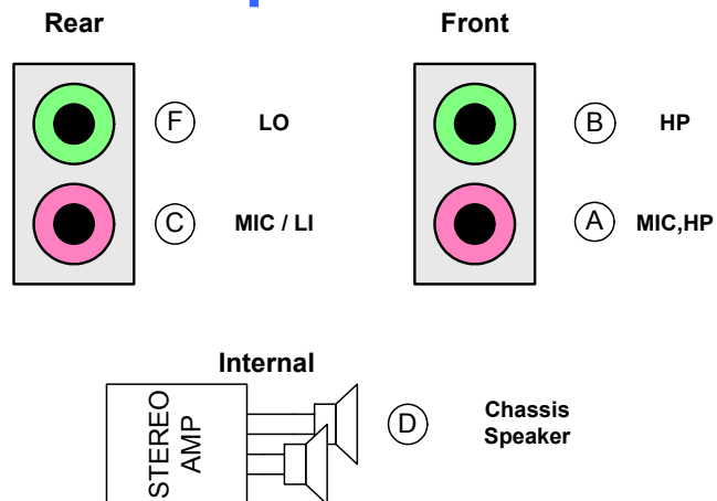
Figure 3. Port Configurations
