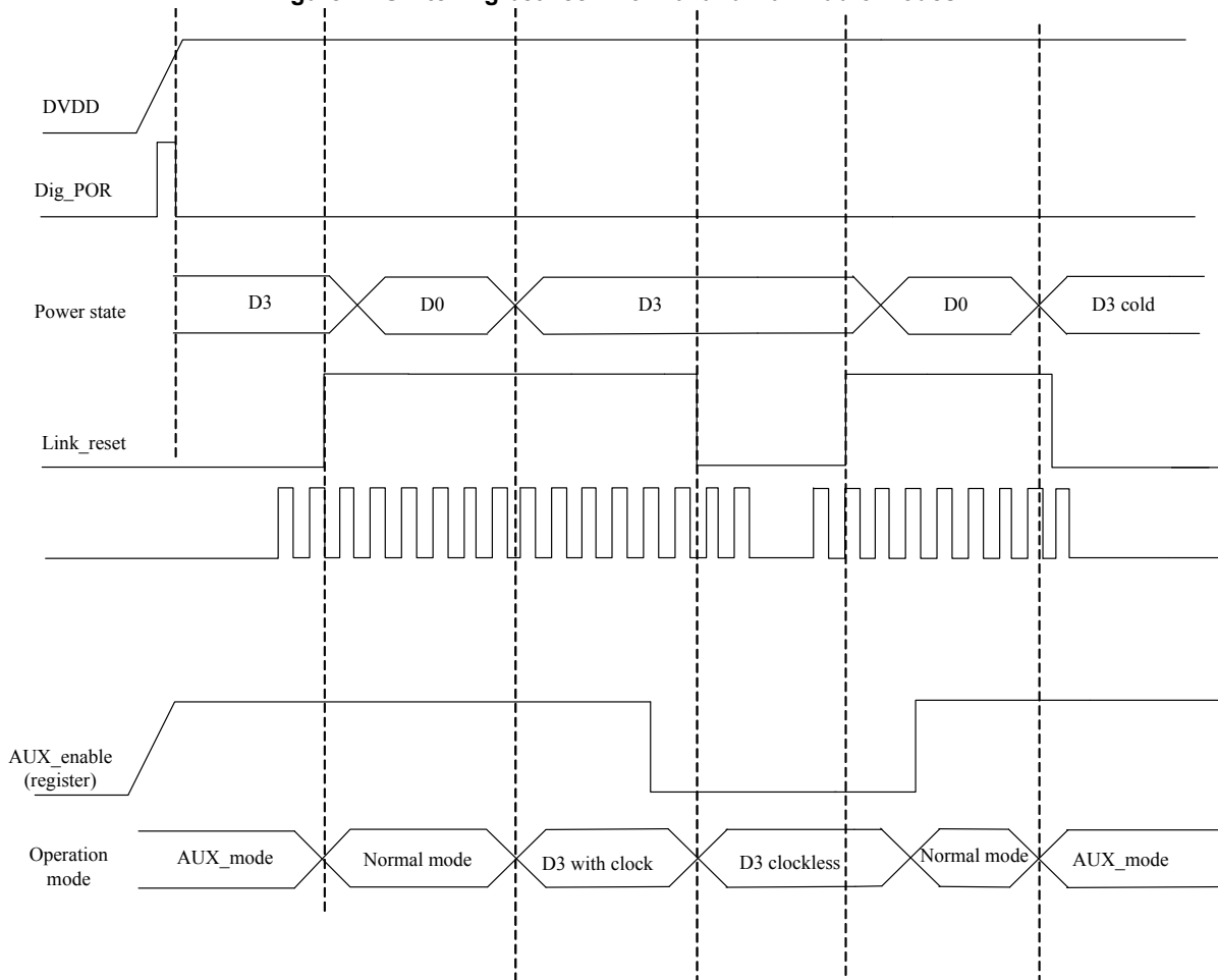
Figure 1. Switching between Normal and Aux Audio Modes
