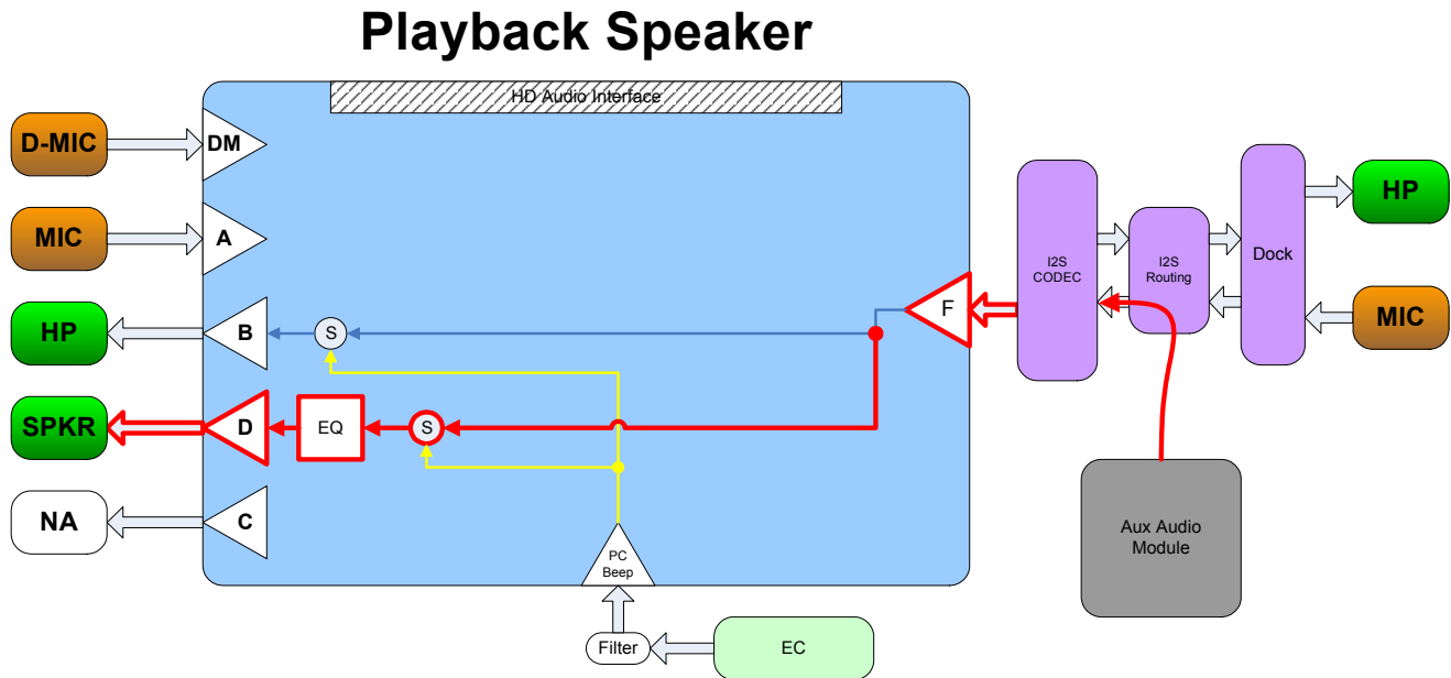
Figure 2. Aux Audio Playback When Nothing Plugged In (or System is not Docked)
