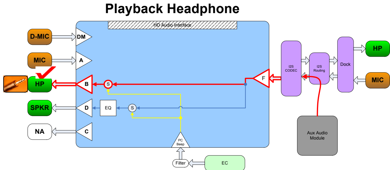
Figure 3. Aux Audio Playback When System Headphones are Plugged In
