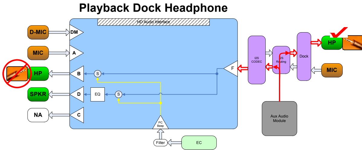
Figure 4. Aux Audio Playback when the System is Docked and Headphones are Plugged In
