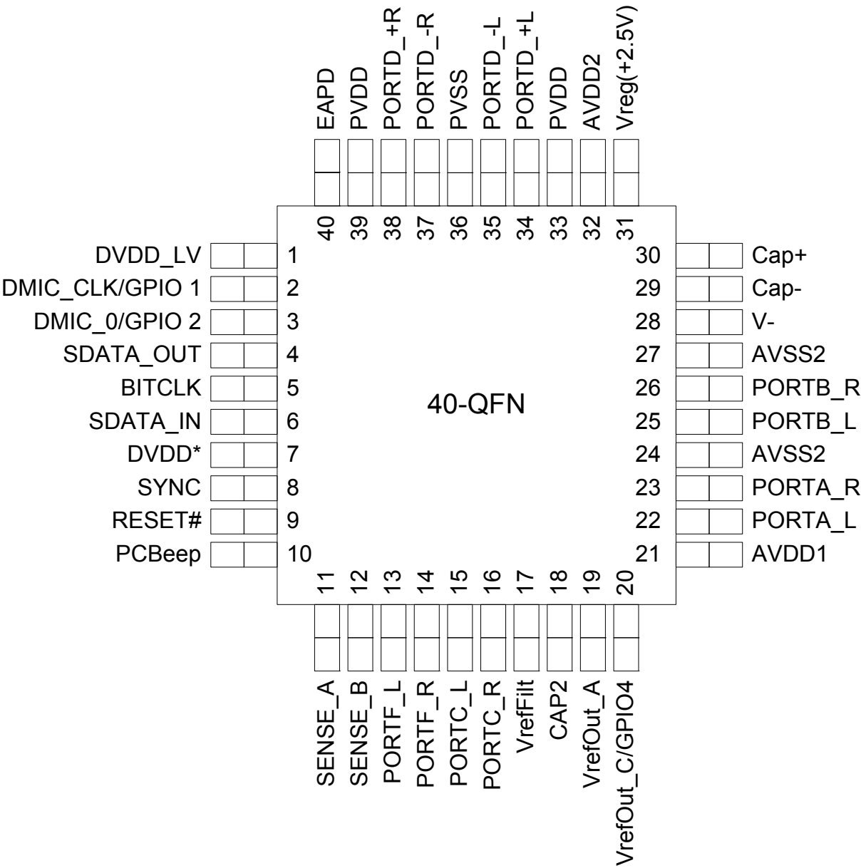
Figure 1. 40QFN Pin Assignment
