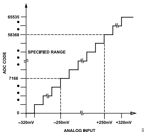
Figure 23. Filtered and Decimated 16-Bit Transfer Function
