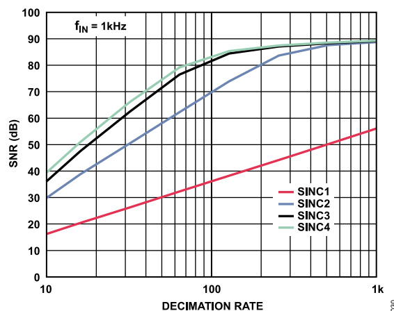
Figure 30. SNR vs. Decimation Rate for Different Sinc Filter Orders
