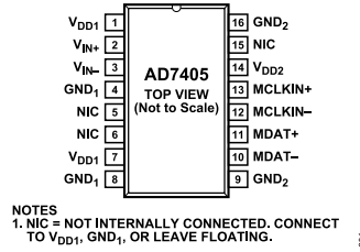
Figure 4. Pin Configuration
