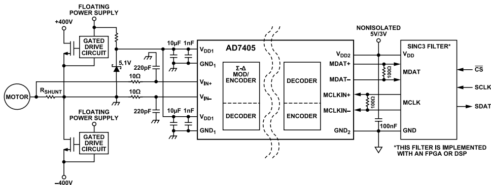
Figure 21. Typical Application Circuit
