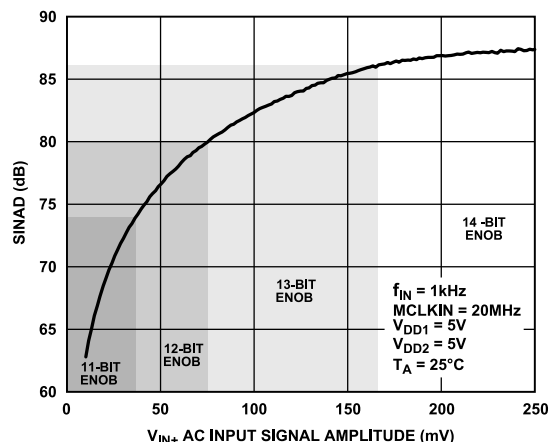
Figure 25. SINAD vs. V_{IN+} AC Input Signal Amplitude
