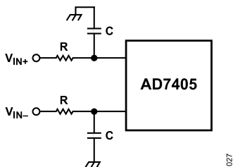
Figure 27. RC Low-Pass Filter Input Network
