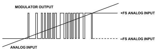
Figure 22. Analog Input vs. Modulator Output
