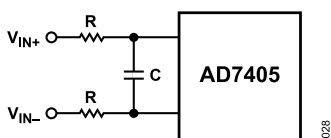
Figure 28. Differential RC Filter Input Network
