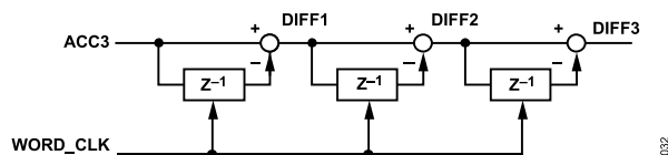
Figure 32. Differentiator
