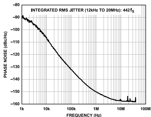
Figure 32. Phase Noise (Absolute) Clock Cleanup; Internal VCO at 1.552 GHz; PFD = 19.44 MHz; LBW = 1.84 kHz; LVPECL Output = 155.52 MHz
