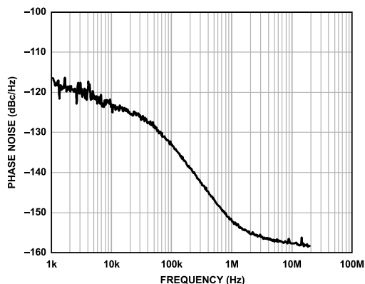
Figure 30. Phase Noise (Absolute) Clock Generation; Internal VCO at 1.475 GHz; PFD = 15.36 MHz; LBW = 40 kHz; LVPECL Output = 122.88 MHz
