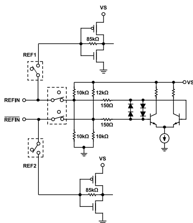
Figure 43. REF IN Equivalent Circuit for Non-XTAL Mode
