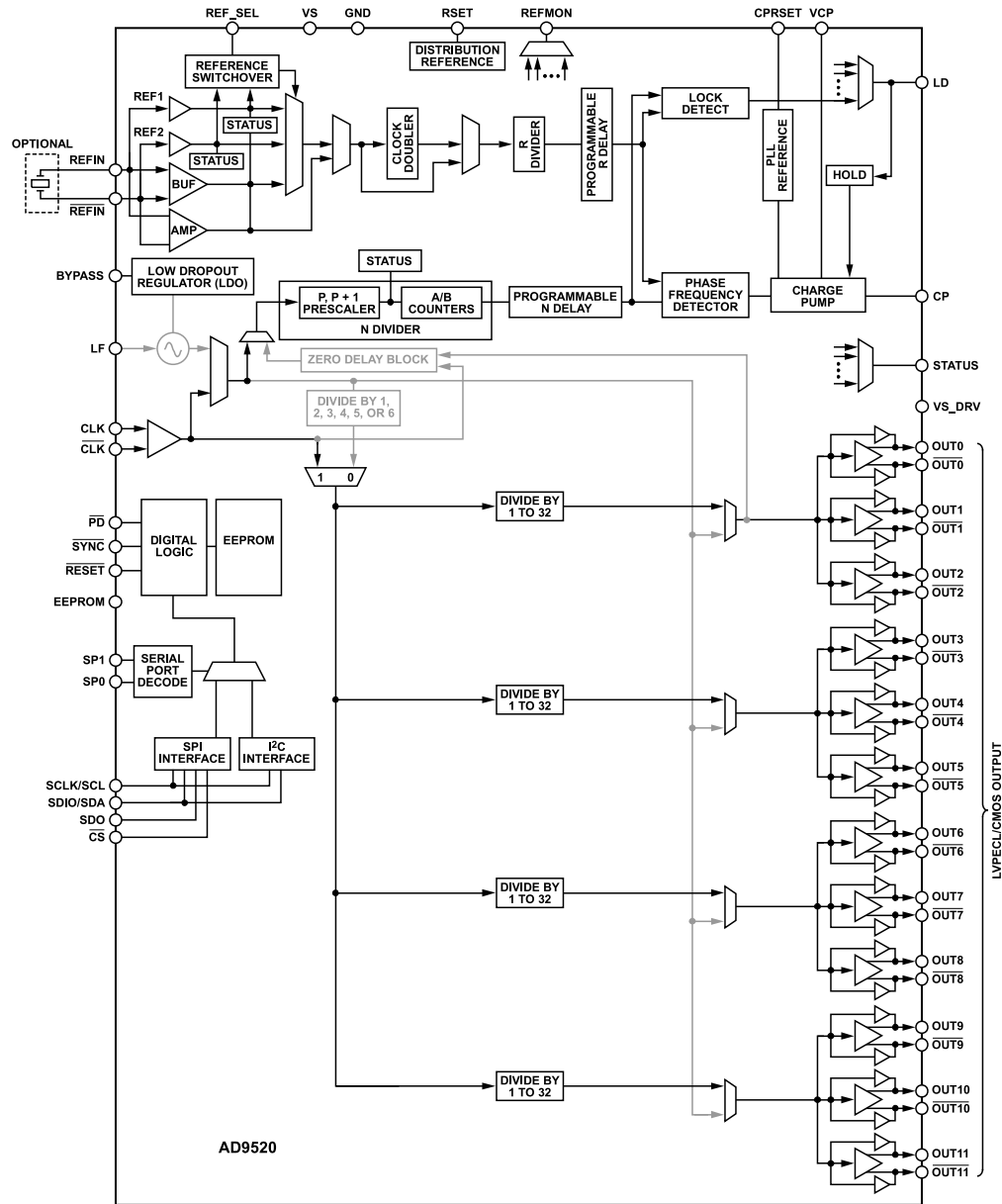
Figure 36. Clock Distribution or External VCO < 1600 MHz (Mode 1)
