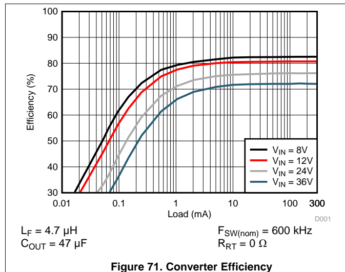
Figure 71. Converter Efficiency
