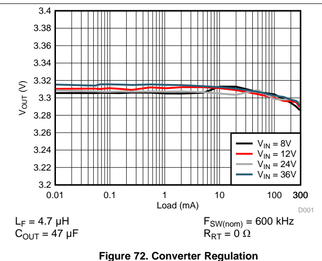
Figure 72. Converter Regulation
