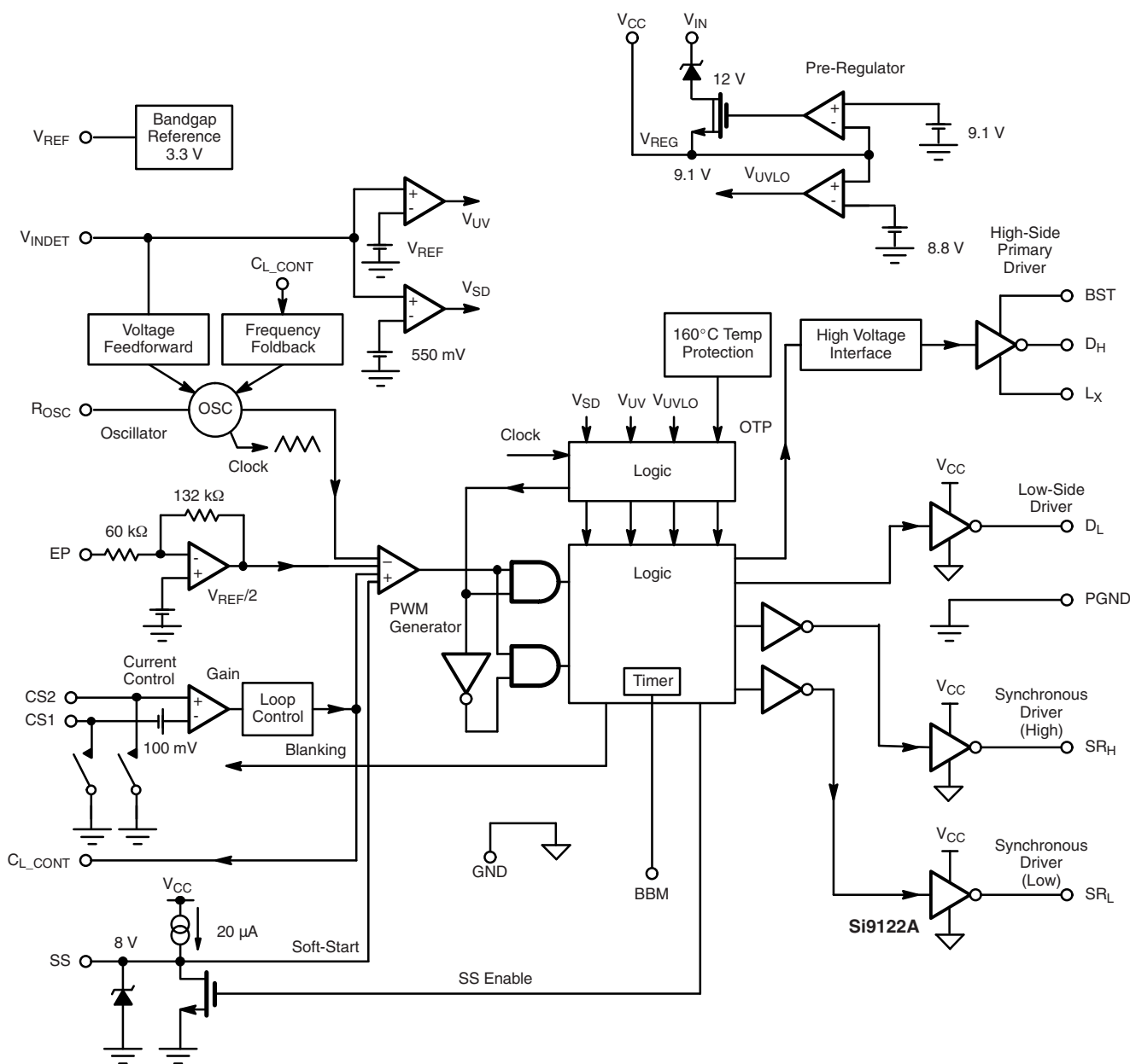
Figure 4. Detailed Si9122A Block Diagram
