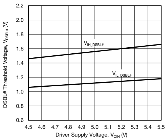
Fig. 21 - DSBL# Threshold vs. Driver Supply Voltage
