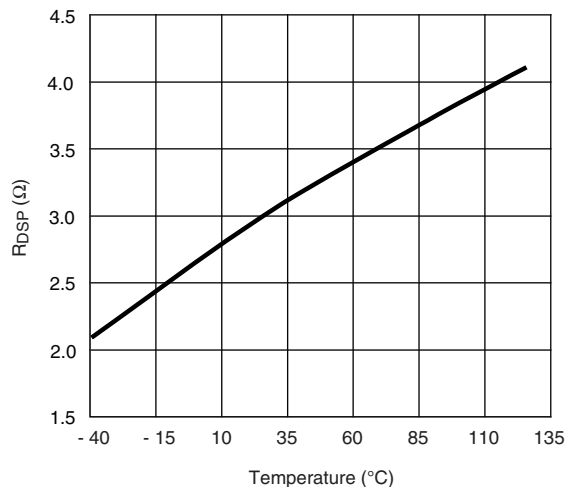
DL R_{DSP} vs. Temperature
