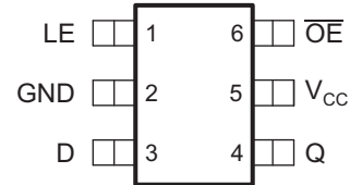
DCK Package 6-Pin SC70 Top View
