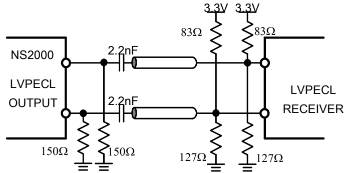
AC-Coupled LVPECL Termination
