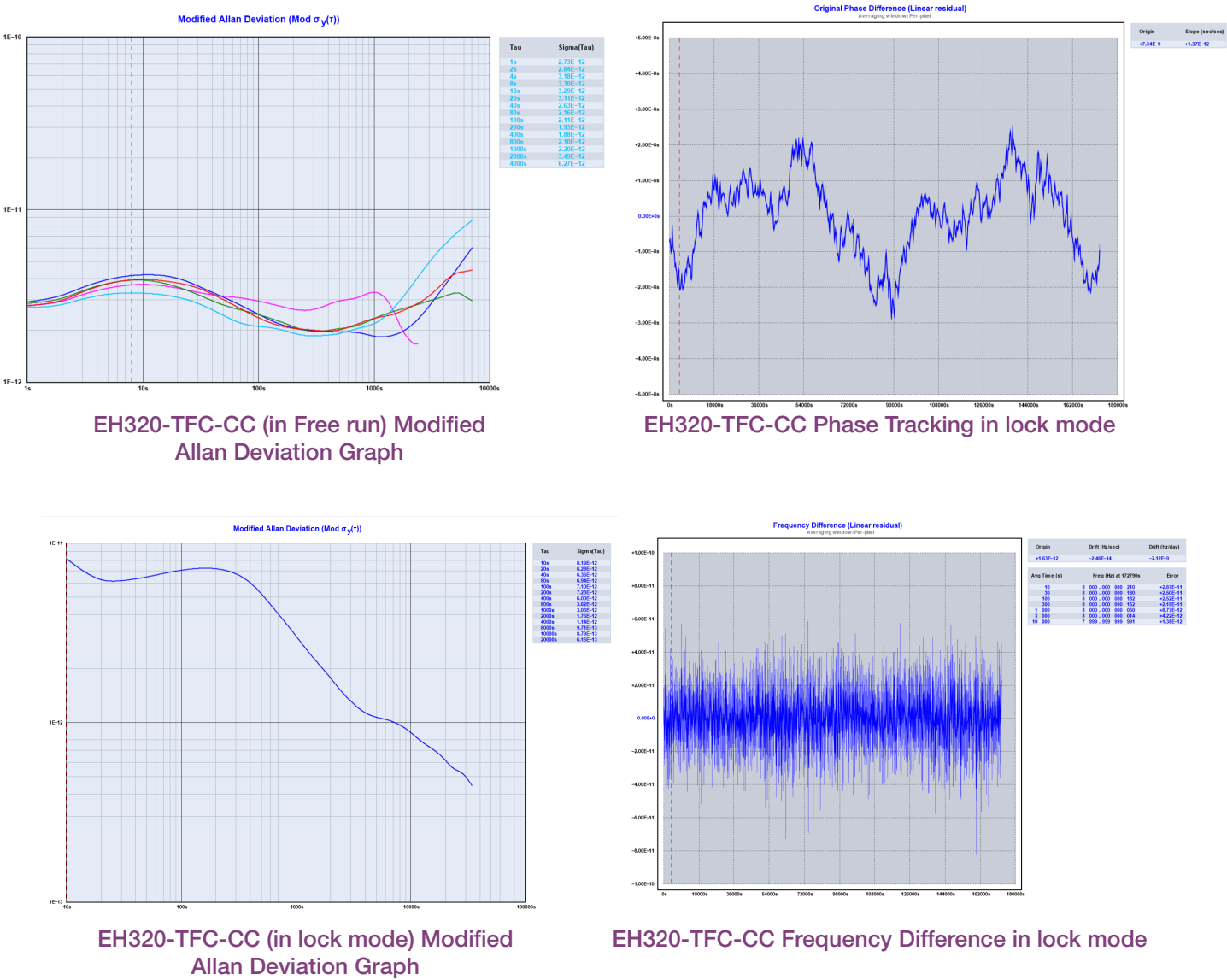
Figure 4: EH320-TFC-CC Performance Comparisons
