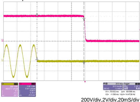
Hold-up time
