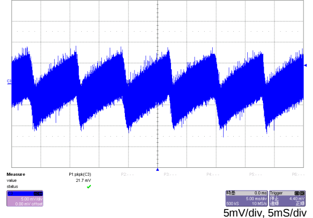
Line frequency ripple(V1)
