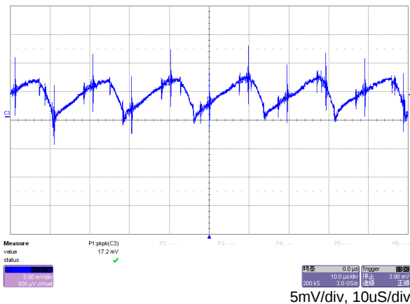
Switching frequency ripple(V1)
