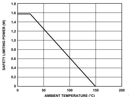
Figure 4. ADuM5028 Thermal Derating Curve, Dependence of Safety Limiting Values with Ambient Temperature per DIN EN IEC 60747-17 (VDE 0884-17)
