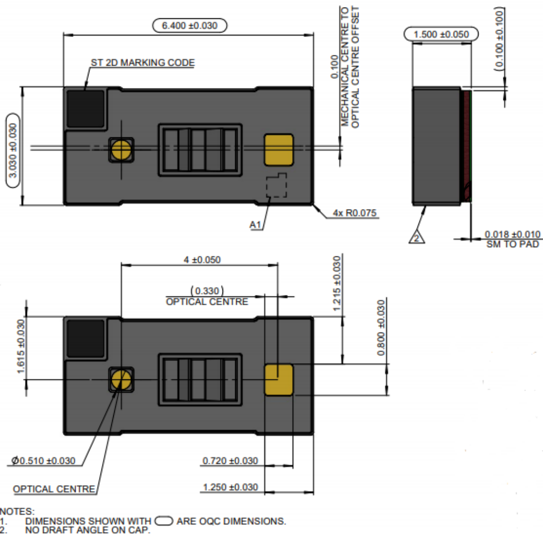
Figure 21. Outline drawing (1/4)
