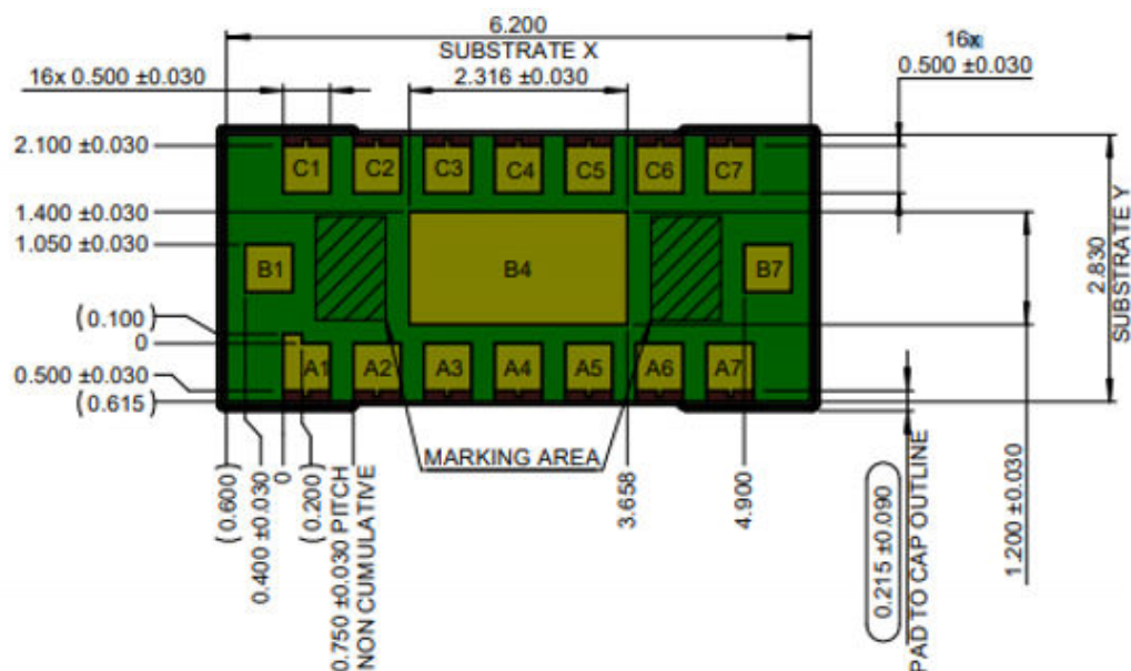
Figure 22. Outline drawing (2/4)
