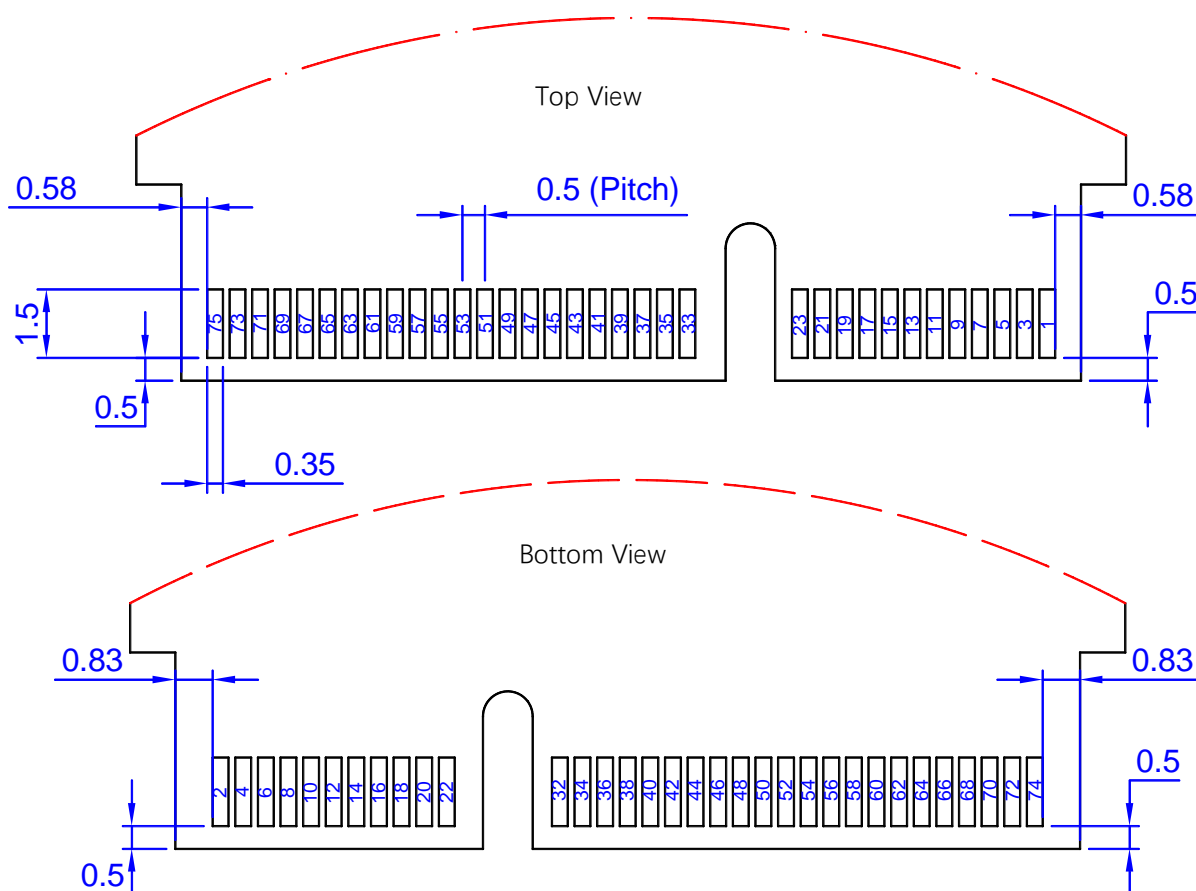
Figure 5-1. Mechanical Drawing of BDE-BW3351NPxM2
