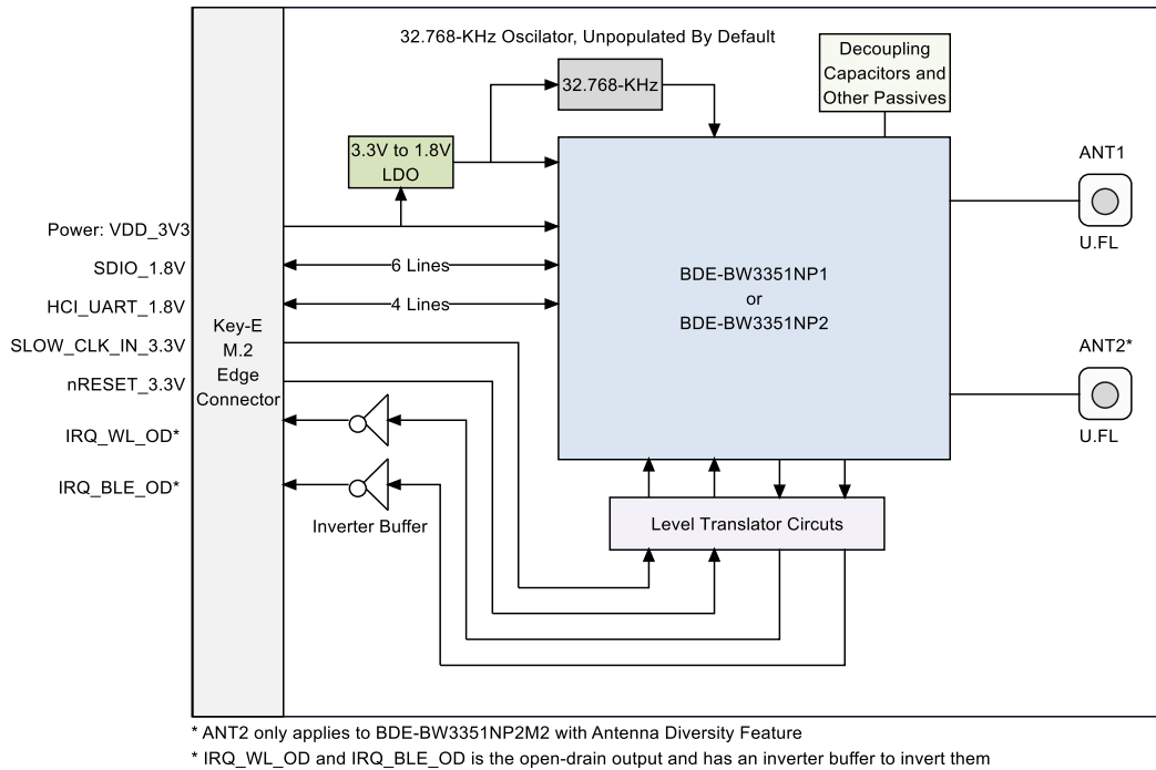
Figure 2-1. Block Diagram of BDE-BW3351NP1M2 or BDE-BW3351NP2M2
