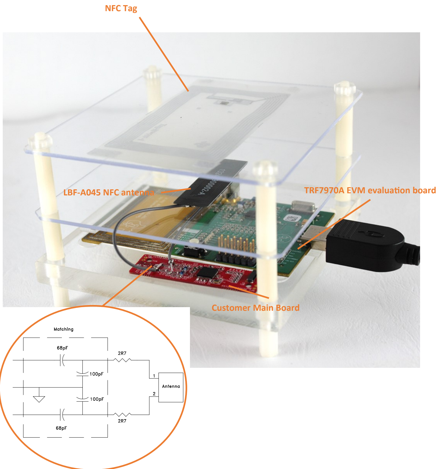
Figure 6. Antenna Test Setup and Matching Circuit
