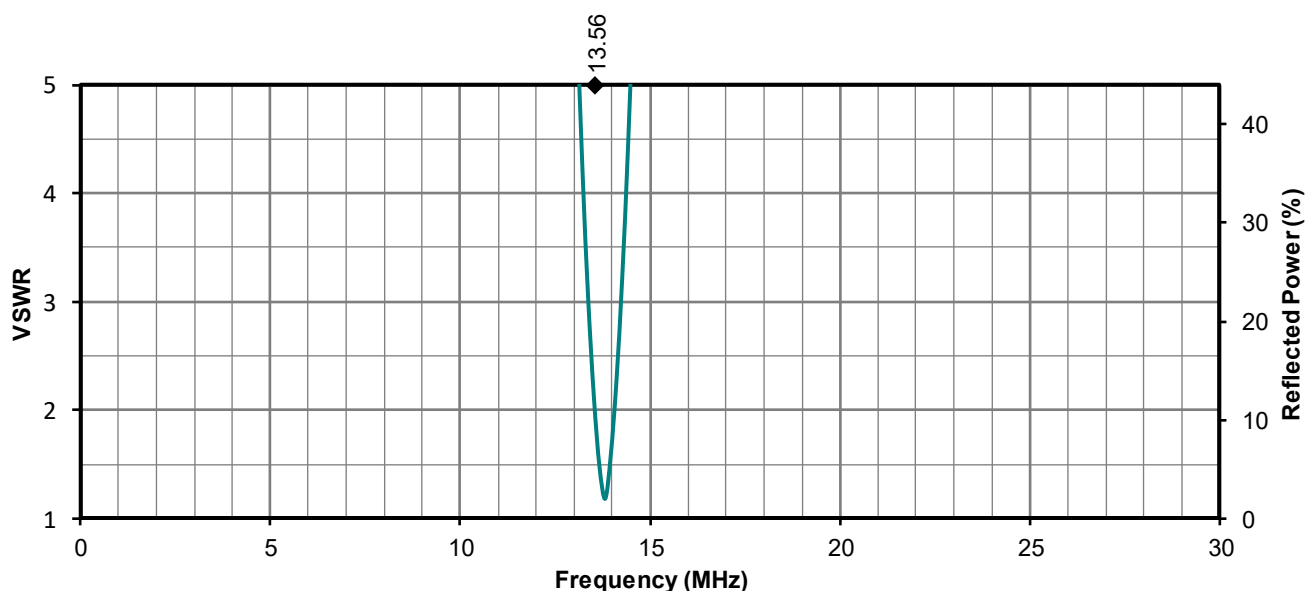
Figure 4. Antenna VSWR, free space
