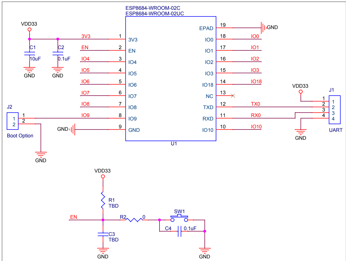
Figure 7: Peripheral Schematics
