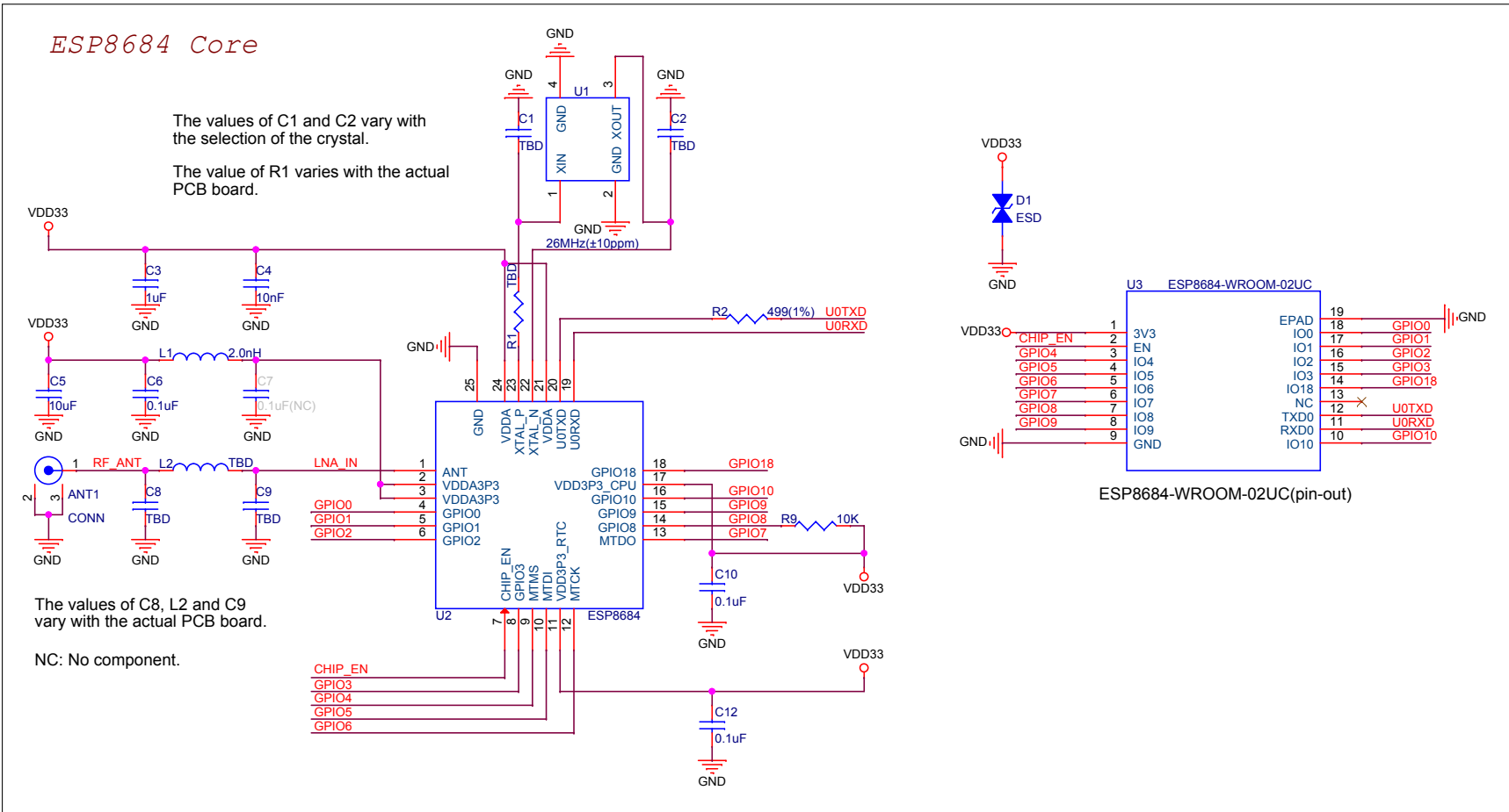
Figure 6: ESP8684-WROOM-02UC Schematics
