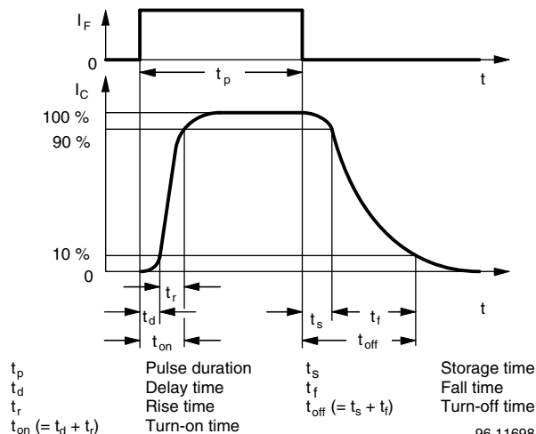
Fig. 4 - Switching Times
