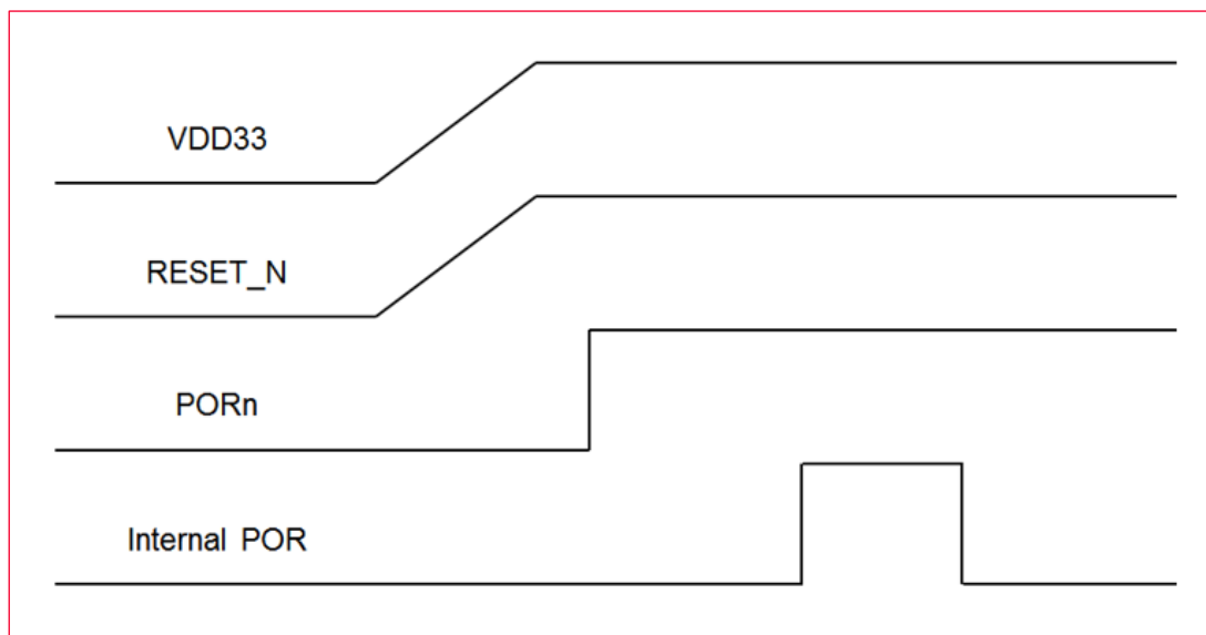
Figure 5: Power-On Sequence
