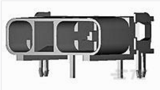
TE Part #2106111-4 Assembly, Right Angle TH Header, 3-Posit
