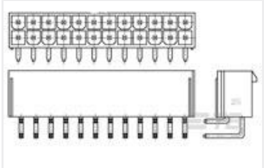
TE Part #1586041-6 6P VAL-U-LOK R/A HDR V2
