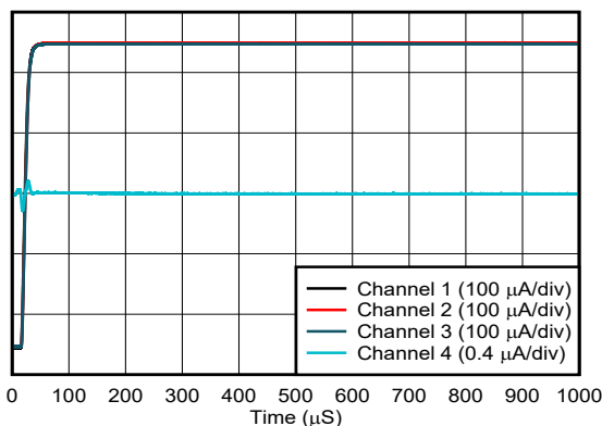
Figure 6-53. Current Output Channel-to-Channel Crosstalk Channel 4 is resident, all other channels are interferers
