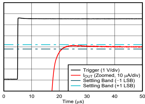
Figure 6-49. Current Output Settling Time: Rising Edge (1/4 to 3/4 scale)
