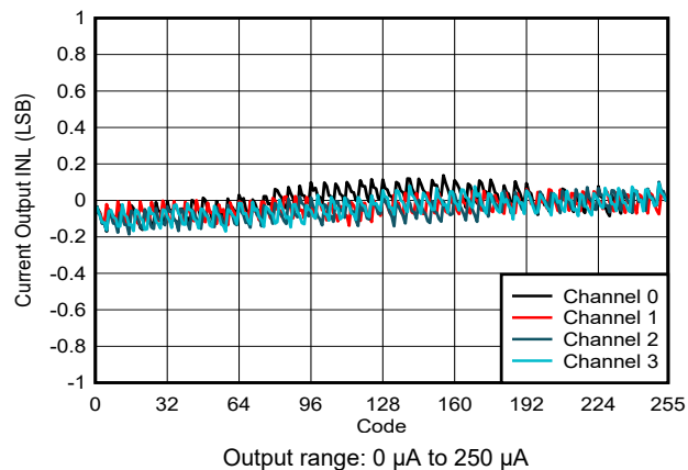
Figure 6-32. Current Output INL vs Digital Input Code
