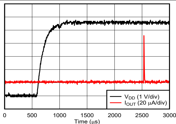
Figure 6-51. Current Output Power-On Glitch DAC at mid scale (0 \mu\text{A} ) stored in EEPROM
